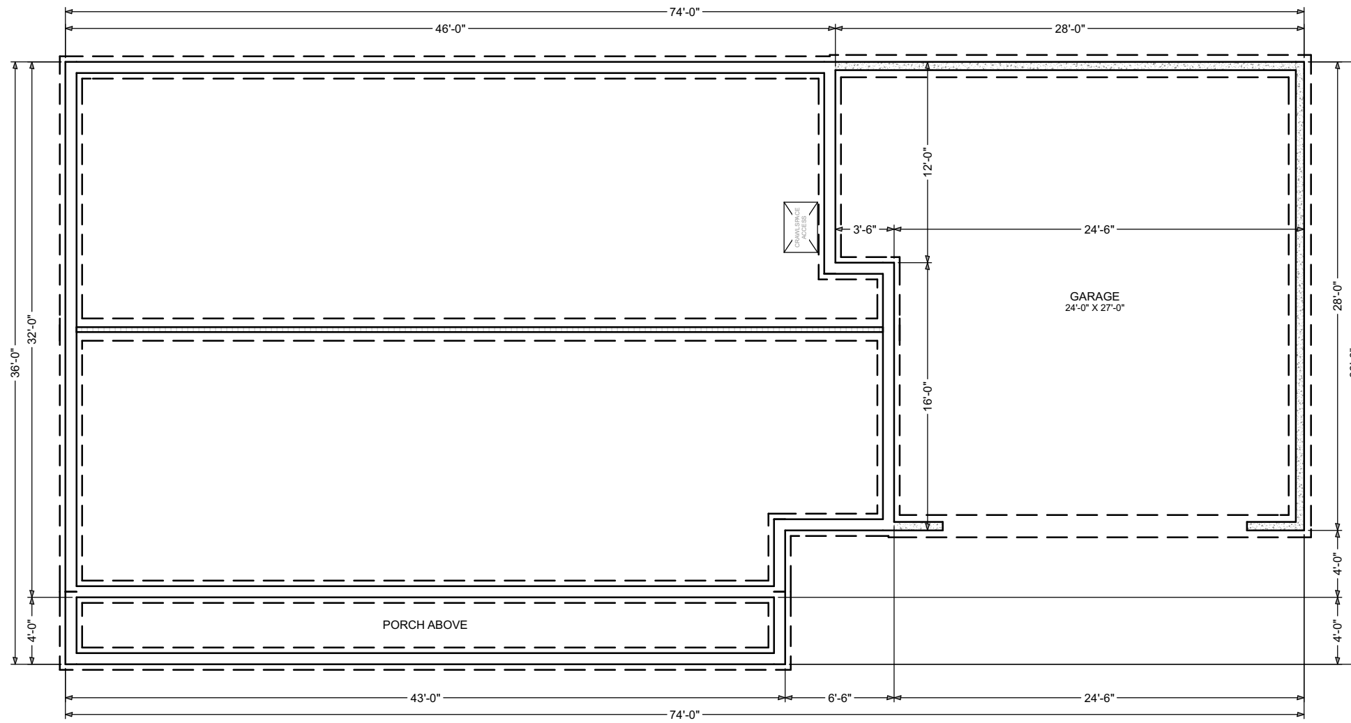
FOUNDATION
