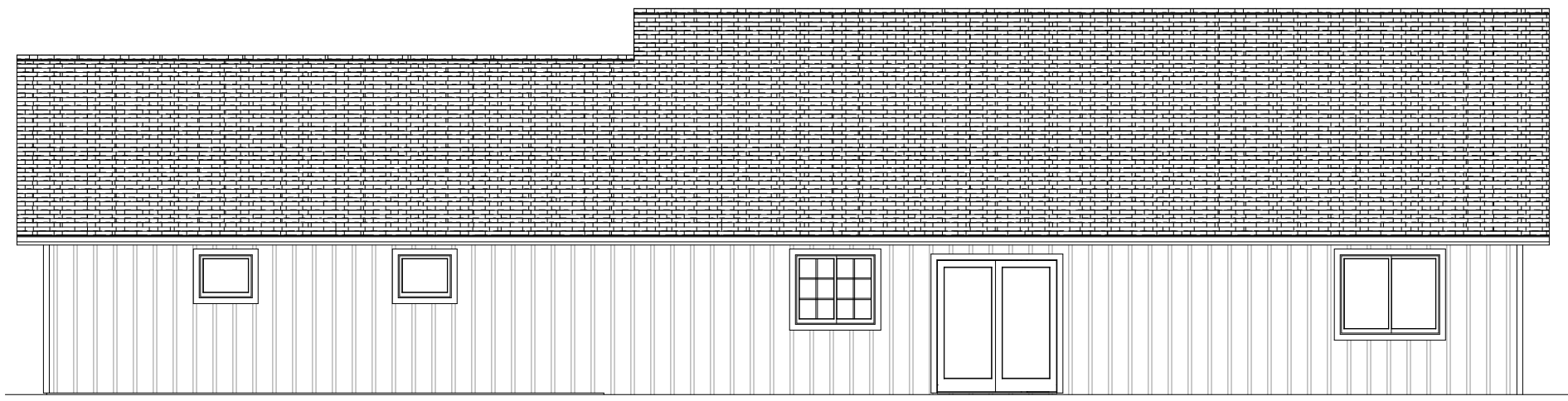
REAR ELEVATION
