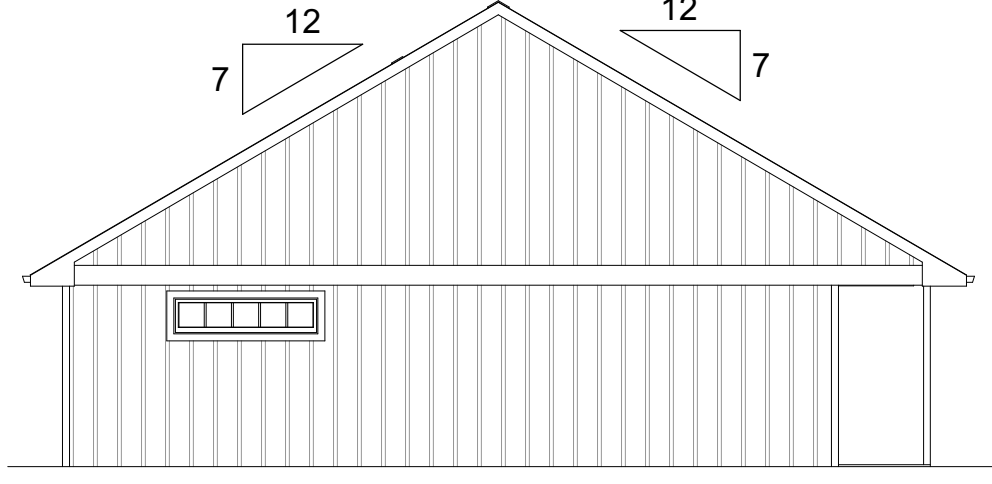
LEFT ELEVATION
