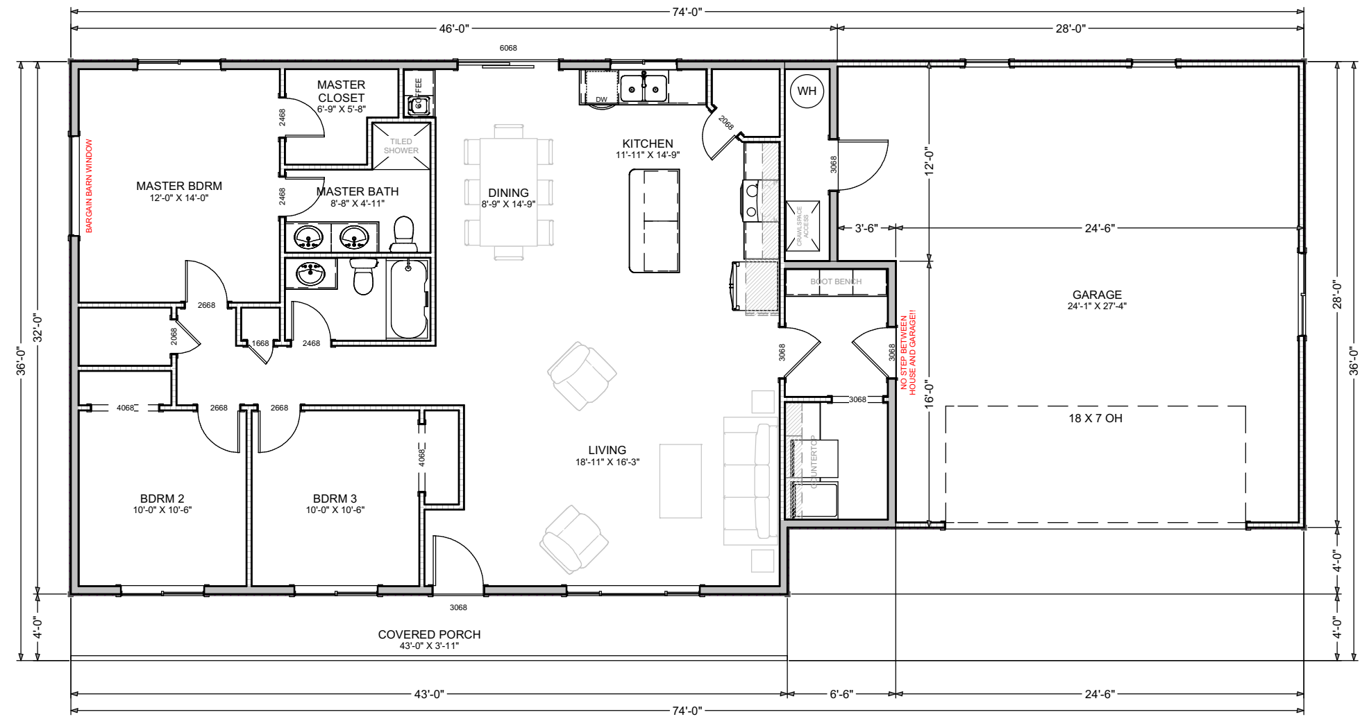
1ST FLOOR
